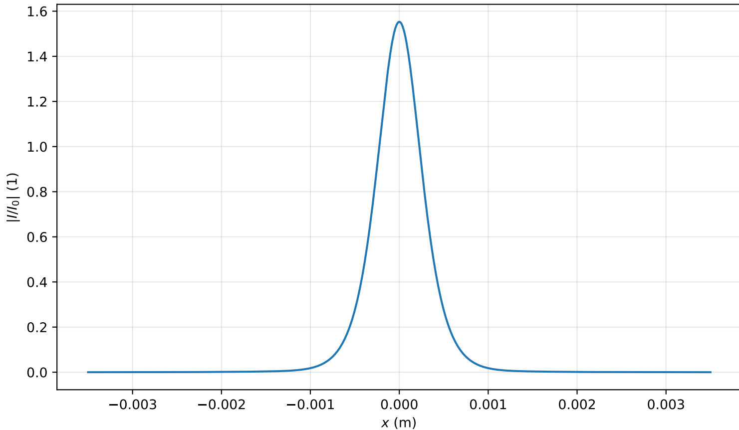
Intensity profile I(x, y = 0, z = 3.105m)/I_0 , P_{in}=0.9P_{cr} , artificial time
